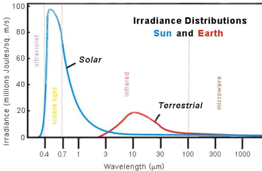
Fig.3. Irradiance distribution of the Sun and Earth
