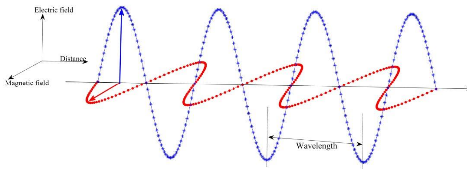
Fig.1. Electromagnetic wave
