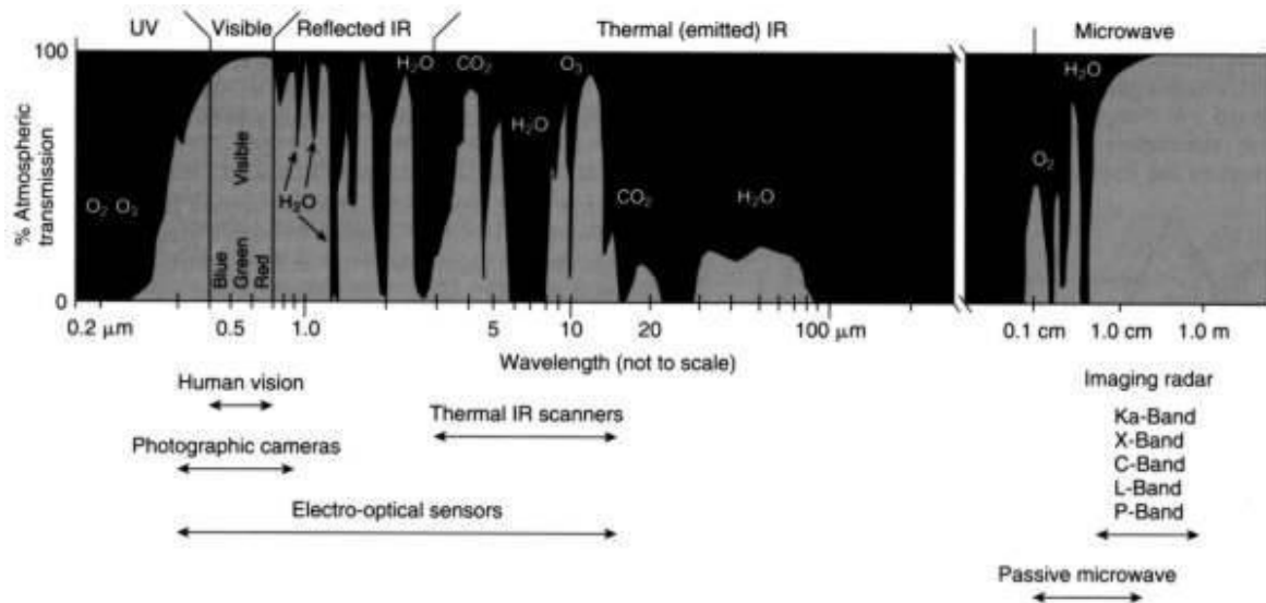
Figure 5. Atmospheric windows in the EMR spectrum
